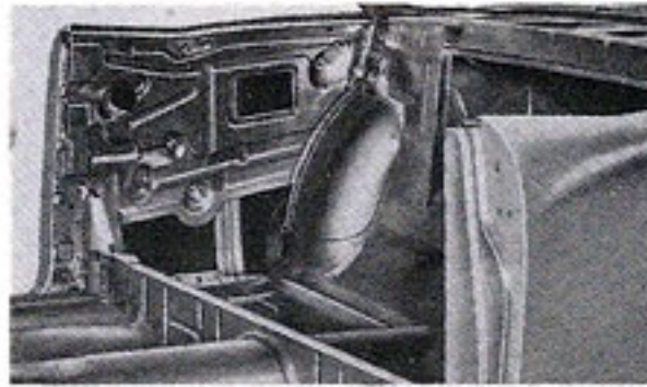
EXTRA REINFORCEMENT IN REAR BODY AREA . . . Husky reinforcements tie the roof rails, package tray, wheelhousings and floor pan into a sturdy, welded assembly. Integral stiffening ribs add rigidity to the domed steel wheelhousings.
